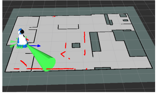
Fig. 4: SocialRobot platform navigating in an indoor office-like scenario, as seen in the ROS visualization tool ( rviz ). Green cones and red dots correspond to sonar and laser range readings respectively.
